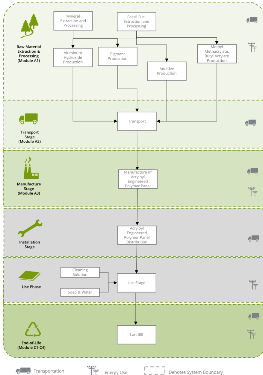
Figure 1. Flow diagram for Acryloyl Engineered Polymer Panel.
